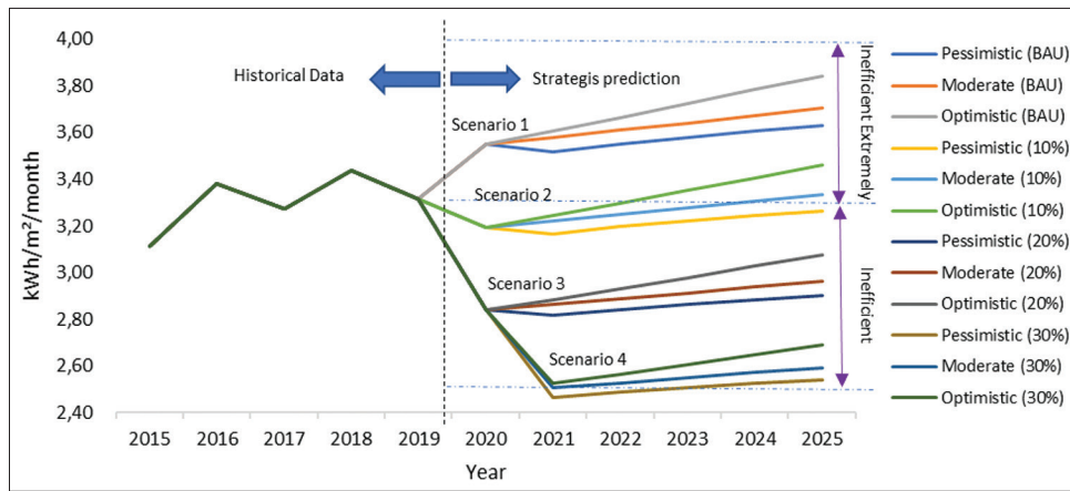
Figure 10: Scenario classification based on EEI standard for area with HVAC system
