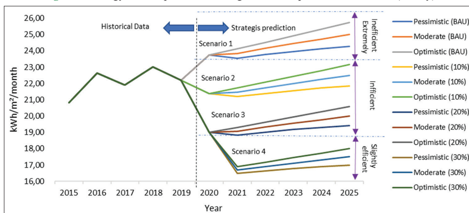
Figure 9: Energy consumption forecasting with load optimization scenario (kWh/y)
