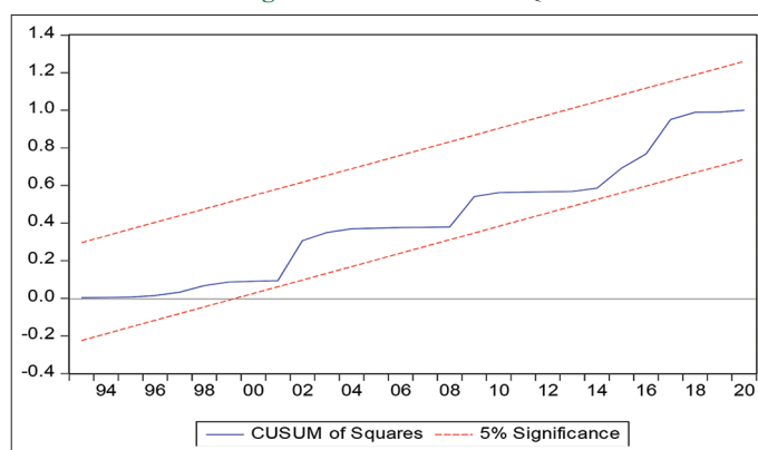
Figure 2: Plot of CUSUMQ
