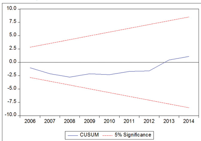
Figure 3: Cumulative sum of recursive residuals test
