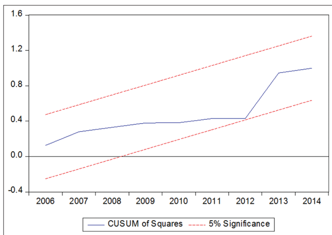
Figure 4: Cumulative sum of recursive residuals of squares test
